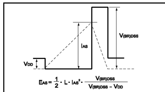
Fig.12 Avalanche Waveform
