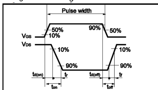
Fig.10 Switching Time Waveform
